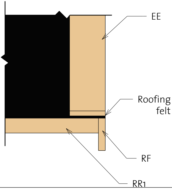
③ Roof Reinforcement
